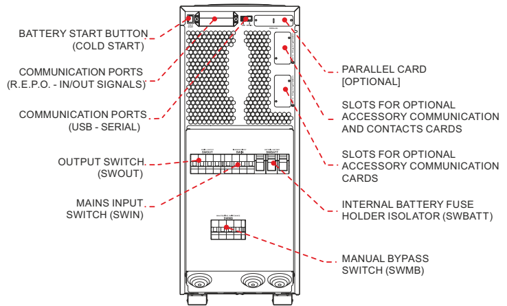
COMPACT 10-20 kVA (rear)
